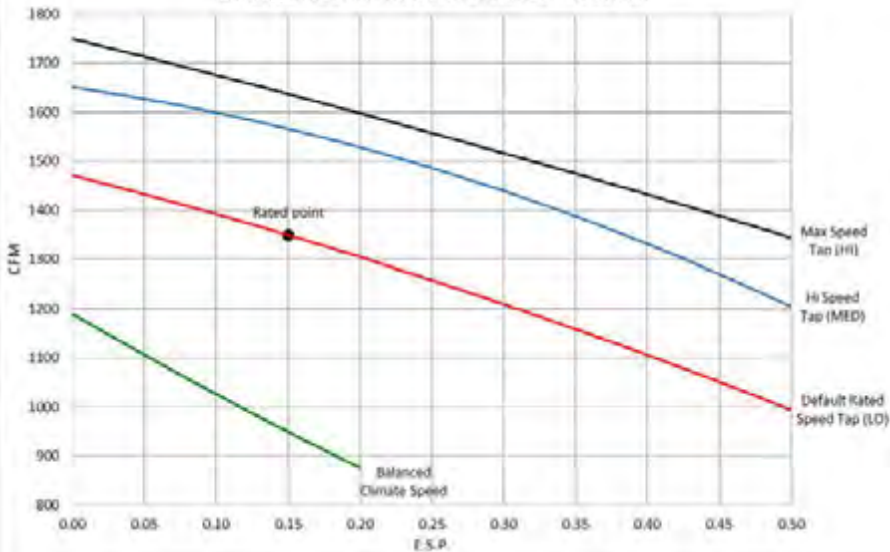
W42A Indoor Airflow Performance - Wet Coil
