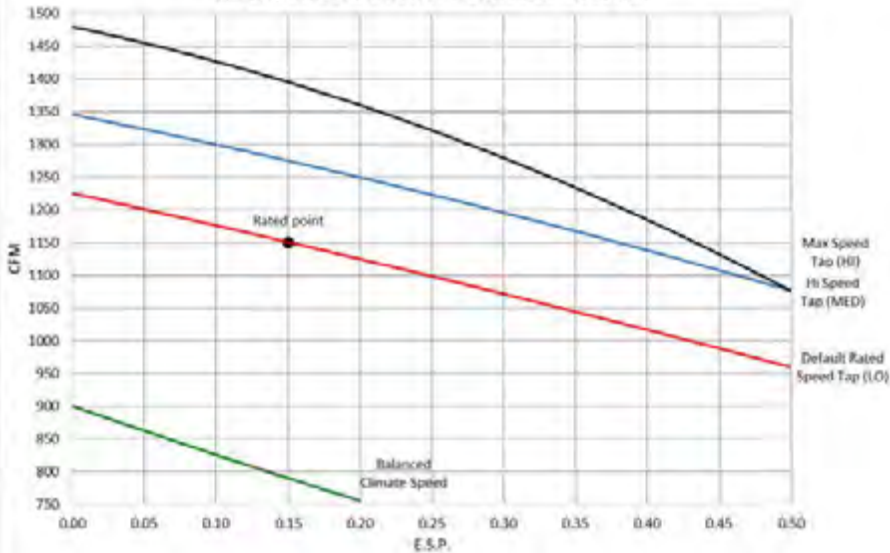
W36A Indoor Airflow Performance - Wet Coil
