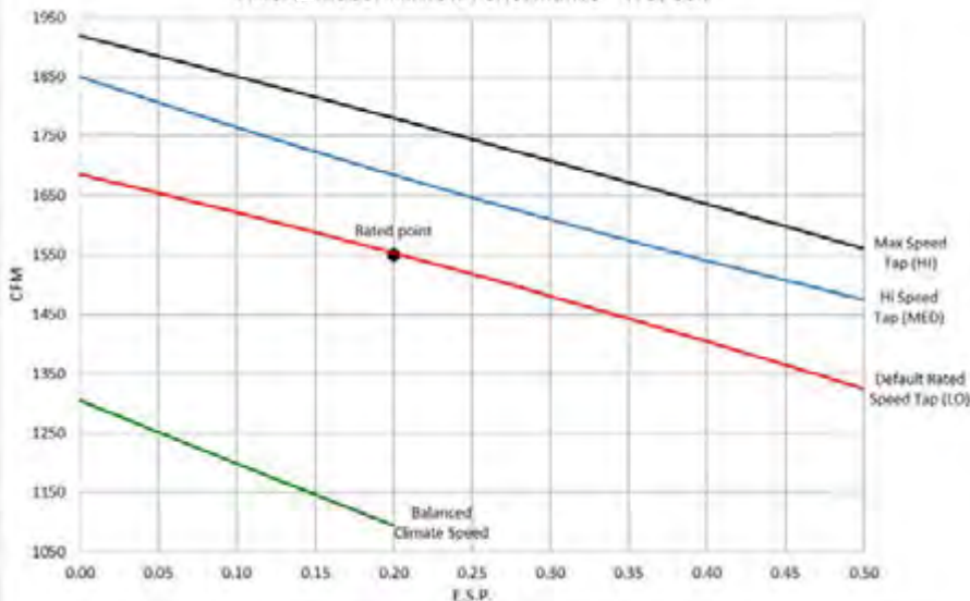
W48A Indoor Airflow Performance - Wet Coil
